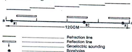
FIGURE 4: Geophysical investigations carried out along section a-a'.
