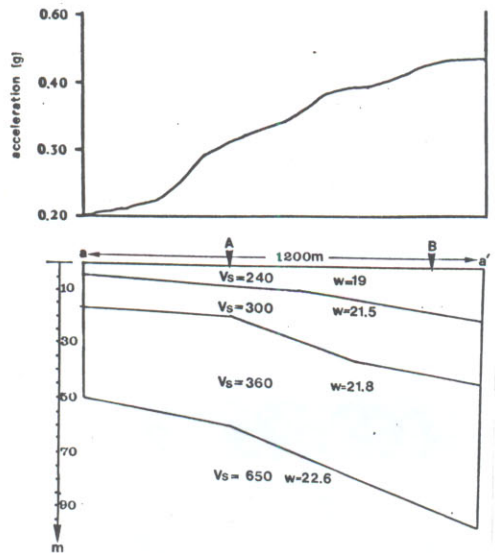
FIGURE 5 : Simplified velocity model of the investigated area. V_s =shear wave velocity in m/s, W is specific weight in \text{KN/m}^3 . Superimposed are also depicted the calculated surface accelerations. Vectors indicate locations where response spectra were derived.
