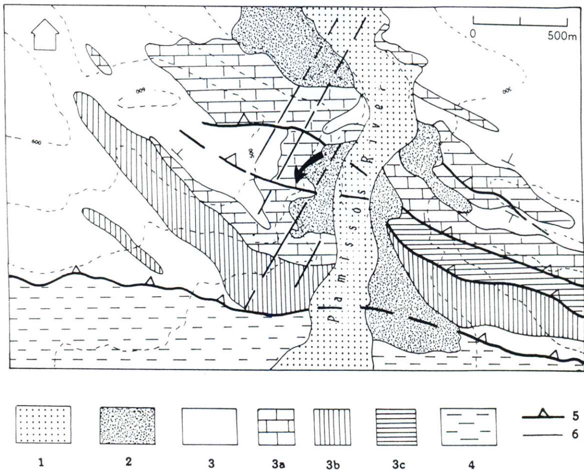
Fig. 2: Northward view of Agriokerasia area (Mouzaki, W. Thessaly), depicting the trace of the thrust along which the cave develops (up) and simplified geological map of the area (down). 1: River deposits, 2: Scree and talus cones, 3: Mouzaki Radiolarites-Pelites formation (Triassic-Jurassic), 3a: Northern Koziakas limestone member, 3b: Agriokerasia Ophiolitic Breccias member, 3c: Vitoumàs limestone member (Up. Triassic), 4: Flysch of W. Thessaly unit (Paleocene - U.Eocene), 5: Thrust, 6: Fault.
