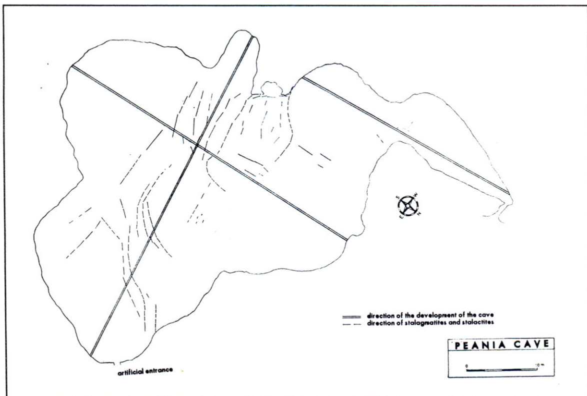
Fig. 4: Plane biew of Koutouki cave (Peania, Attica) and the direction of the development of it, in accordance with the main joint sets (after DERMITZAKIS & LEKKAS, 1977).
